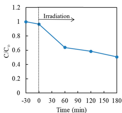
Figure 3. Effect of time on the photocatalytic reduction of Cr(VI) in aqueous solution with P25 TiO 2 . Cr(VI) sample: 30 \mu\text{g}\cdot\text{mL}^{-1} (30 mL); TiO 2 : 20 mg (0.67 \text{mg}\cdot\text{mL}^{-1} ).
