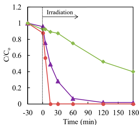
Figure 5. Effect of different commercial TiO_2 on the photocatalytic treatment of Cr(VI) with nanoparticles of TiO_2 in an aqueous solution, in the presence of formic acid hole scavenger. Cr(VI) sample: 30 \mu\text{g}\cdot\text{mL}^{-1} (30 mL); TiO_2 : 20 mg ( 0.67 \text{ mg}\cdot\text{mL}^{-1} ). Circle (red): Ishihara Sangyo ST-01; triangle (purple): AEROXIDE ® P25 TiO_2 ; diamond (green): FUJIFILM Wako Pure Chemical Corp.
