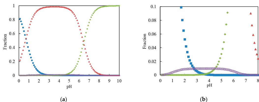
Figure 1. (a) Distribution of Cr(VI) species as functions of pH. Square (blue): \text{H}_2\text{CrO}_4 ; triangle (red): \text{HCrO}_4^- ; diamond (green): \text{CrO}_4^{2-} ; circle (purple): \text{Cr}_2\text{O}_7^{2-} ; (b) Magnification for \text{Cr}_2\text{O}_7^{2-} species.
