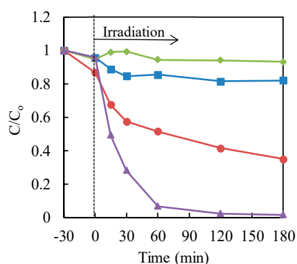
Figure 4. Effect of the hole scavengers on the photocatalytic reduction of Cr(VI) in aqueous solution with P25 TiO 2 . Cr(VI) sample: 30 \mu\text{g}\cdot\text{mL}^{-1} (30 mL); TiO 2 : 20 mg (0.67 \text{mg}\cdot\text{mL}^{-1} ). Triangle (purple): TiO 2 with formic acid (3000 \mu\text{g}\cdot\text{mL}^{-1} ); circle (red): TiO 2 with ammonium formate (3000 \mu\text{g}\cdot\text{mL}^{-1} ); square (blue): formic acid (3000 \mu\text{g}\cdot\text{mL}^{-1} ) only; diamond (green): ammonium formate (3000 \mu\text{g}\cdot\text{mL}^{-1} ) only.
