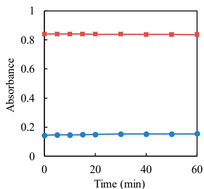
Figure 2. Effect of standing time on the absorbance of the complex between Cr(VI) and 1,5-diphenylcarbazide. Cr(VI) concentration: Circle (blue) 10 \mu\text{g}\cdot\text{mL}^{-1} ; square (red): 50 \mu\text{g}\cdot\text{mL}^{-1} .
