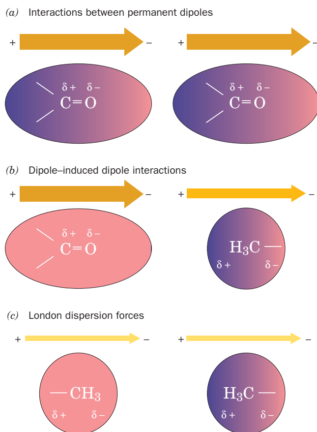
Figure 2-5 | Dipole–dipole interactions.
